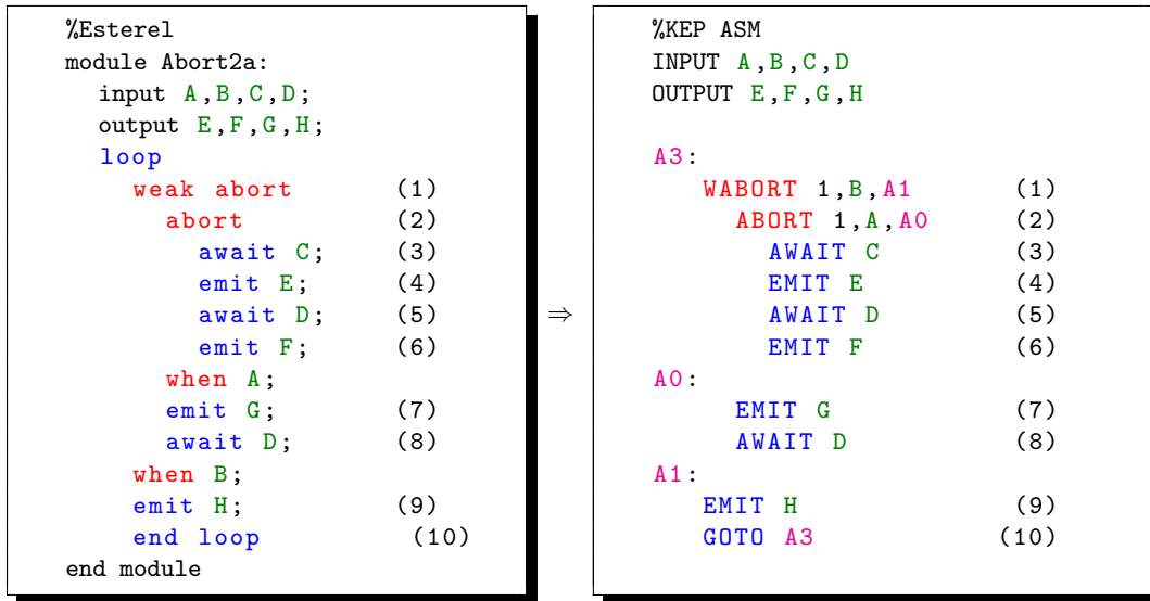
Fig. 8. The program of example Abort2a
