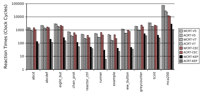
Fig. 9. The worst-/average-case reaction times (in clock cycles) for the KEP and MicroBlaze implementations. Note the logarithmic scale.
