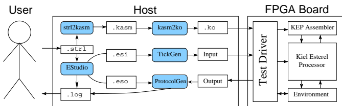
Fig. 7. The KEP evaluation platform.
