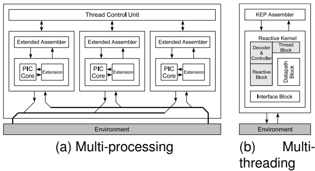
Fig. 2. Comparison of concurrent reactive architectures.
