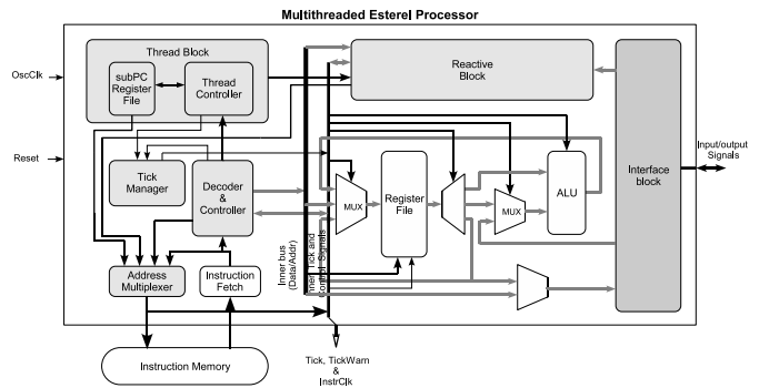
Fig. 3. Overview of the KEP architecture.
