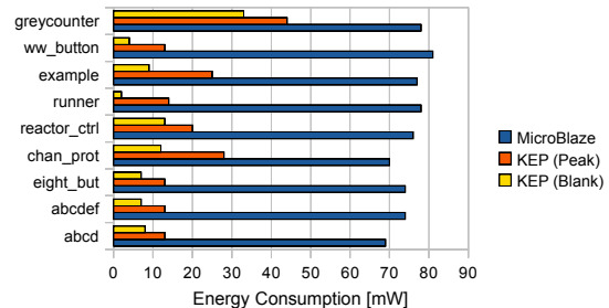
Fig. 10. Energy consumption of KEP and MicroBlaze.
