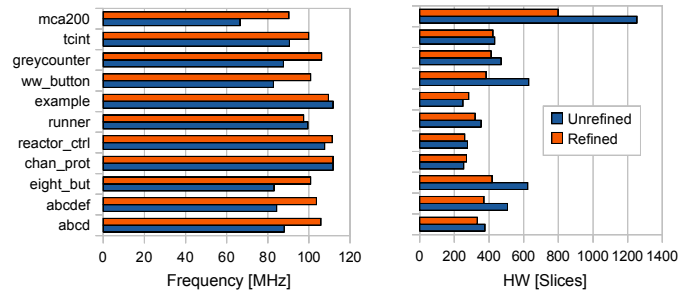
Fig. 8. Clock frequencies and hardware costs with and without ISA refinement.
